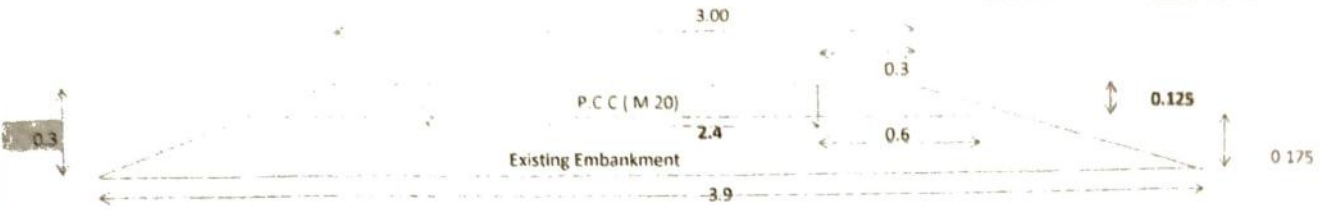
SECTIONAL ELEVATION
